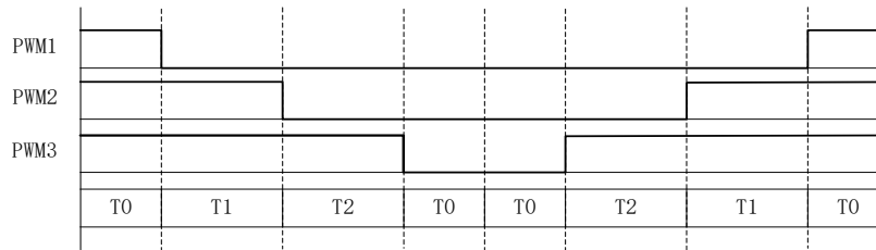
Figure 12-8 Continuous SVPWM Output Waveform
