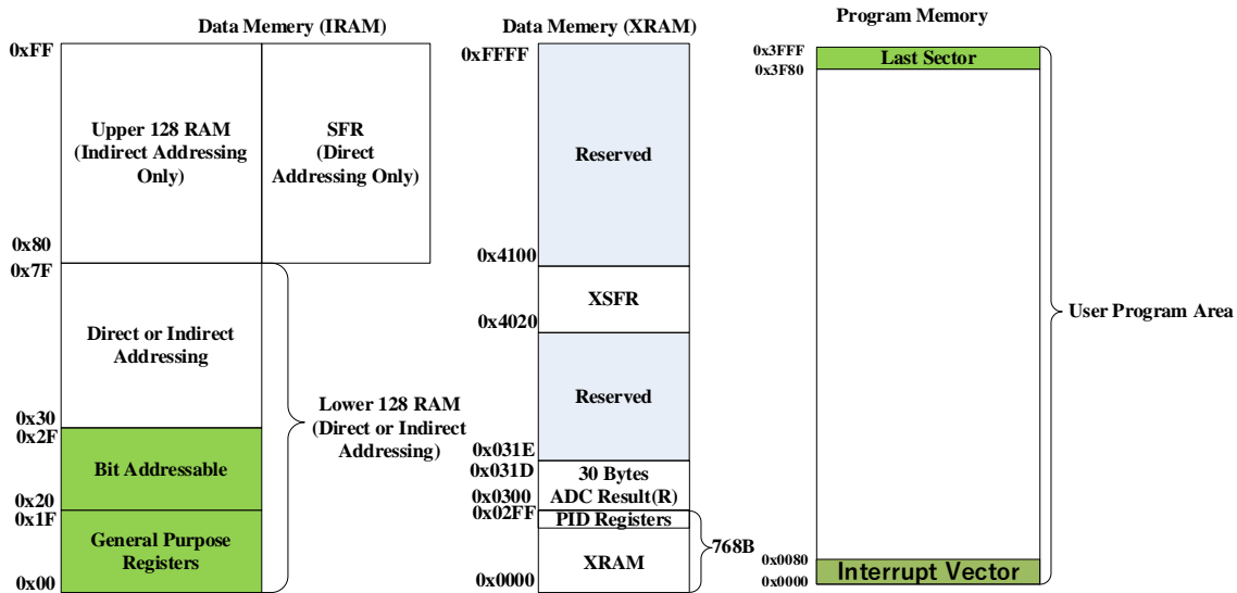
Figure 1-2 Memory Organization
