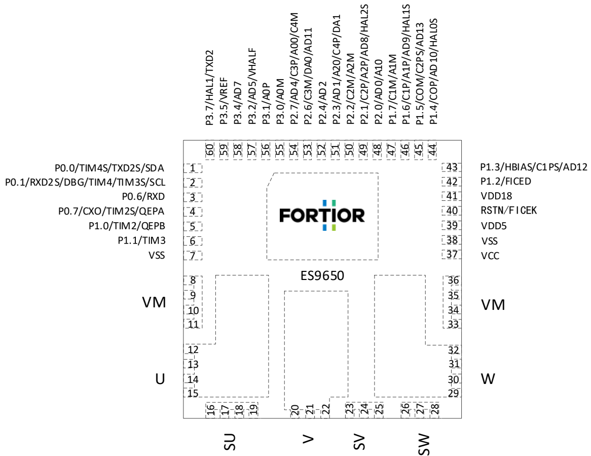
Figure 2-1 ES9650 QHF8080-60L Pinout Diagram
