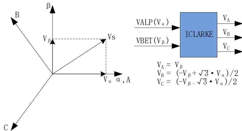
Figure 12-3 Inverse Clarke Transformation
