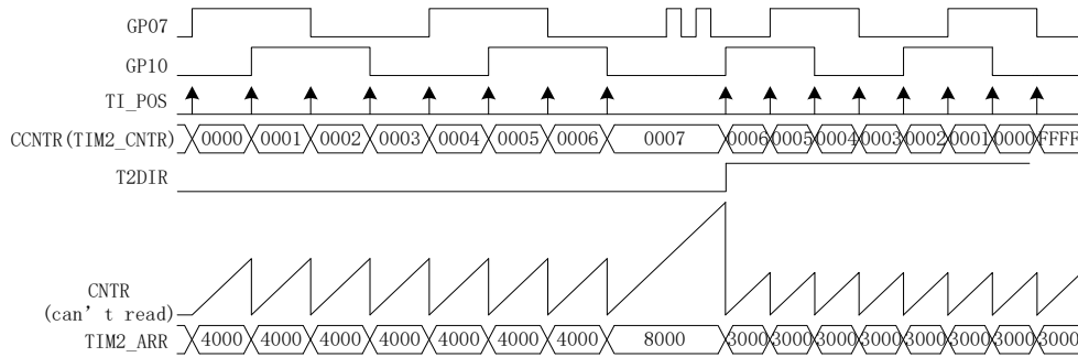
Figure 14-10 Timing Diagram of QEP & RSD Mode
