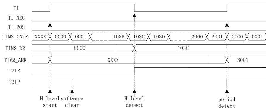
Figure 14-6 Timing Diagram of Input Capture Mode ( T2CES = 0 )
