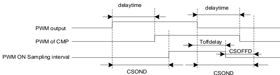
Figure 14-11 PWM ON Sampling mode
