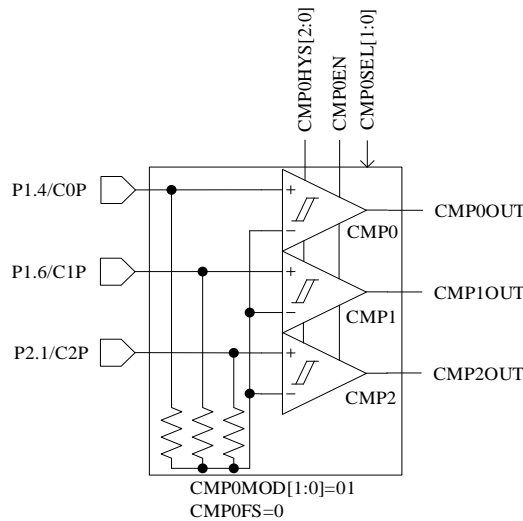
Figure 27-9 CMPG Mode with Built-in Three Comparators and Resistors (without Functional Switching)
