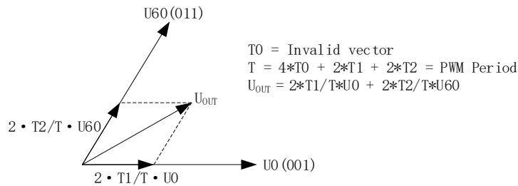
Figure 12-7 Voltage Vector Synthesis
