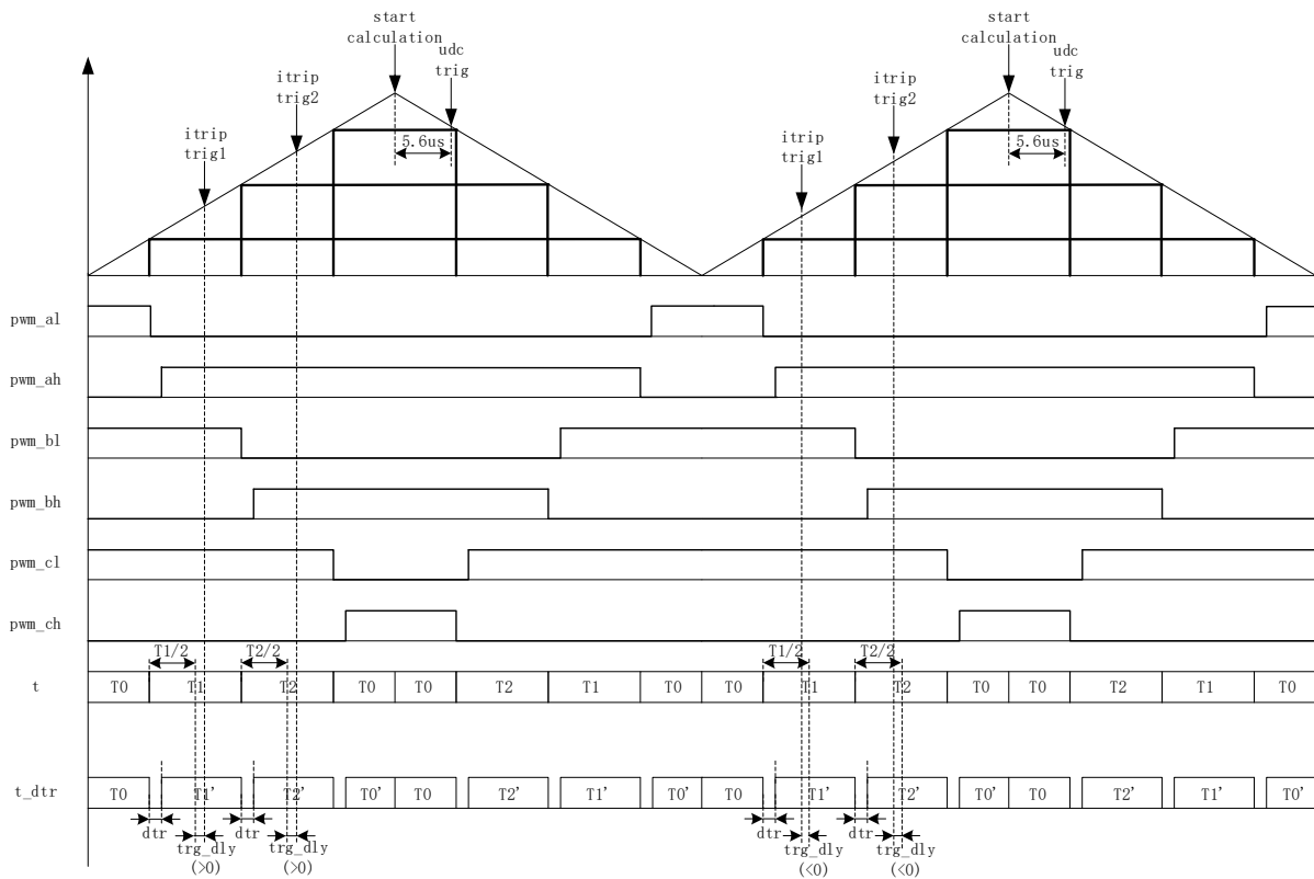
Figure 12-10 Single-shunt Current Sampling Timing Diagram
