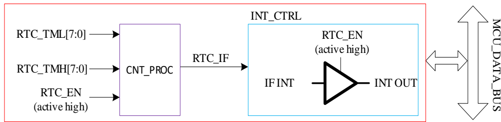
Figure 19-1 RTC Functional Block Diagram
