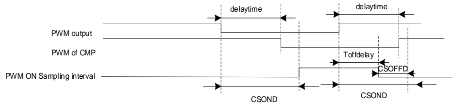
Figure 27-14 PWM OFF Sampling Mode
