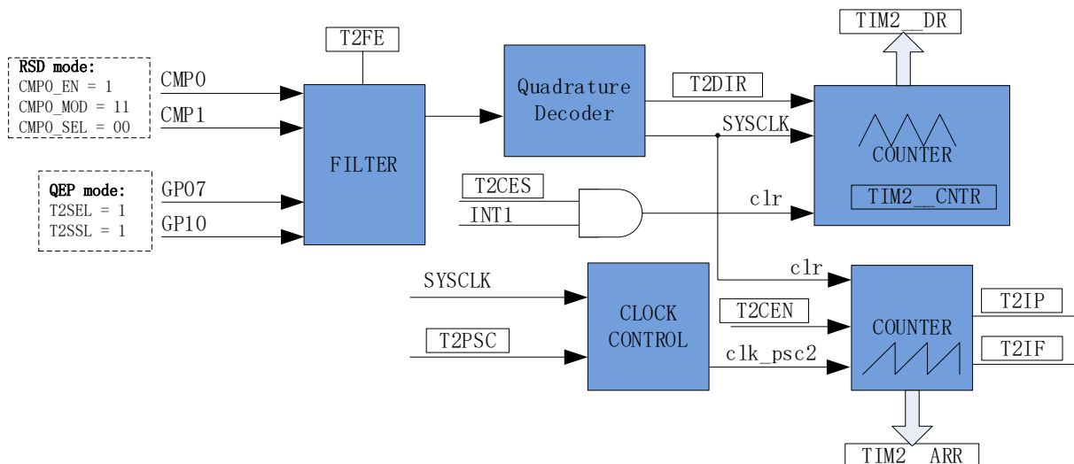
Figure 14-9 Schematic Block Diagram of QEP & RSD Mode
