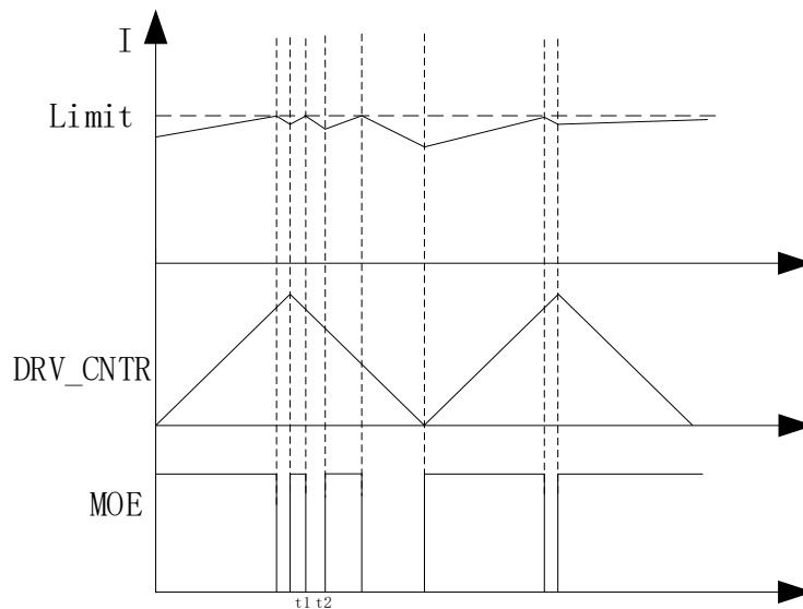
Figure 27-6 Cycle-by-Cycle Current Limiting Waveform ( t_2 - t_1 = 5\mu s ) when EVT\_FILT[MOEMD] = 11
