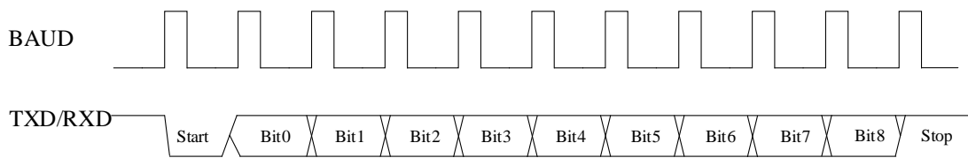
Figure 9-4 UART Communication Timing Diagram
