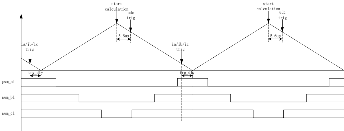
Figure 12-13 Dual/Triple-Shunt Alternating Current Sampling Mode
