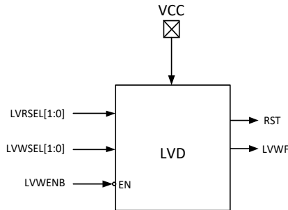
Figure 28-3 LVD Module
