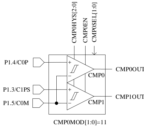
Figure 27-12 CMPG Mode with Two Comparators
