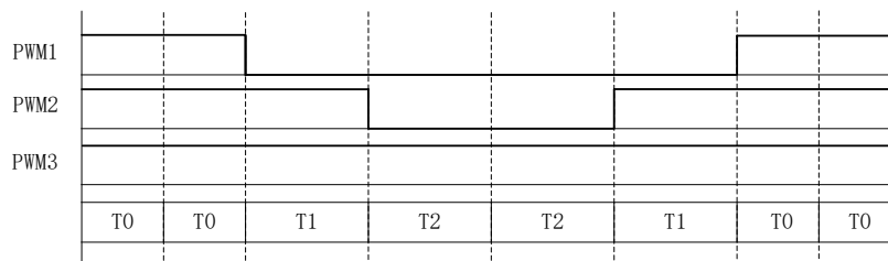
Figure 12-9 Discontinuous SVPWM Output Waveform
