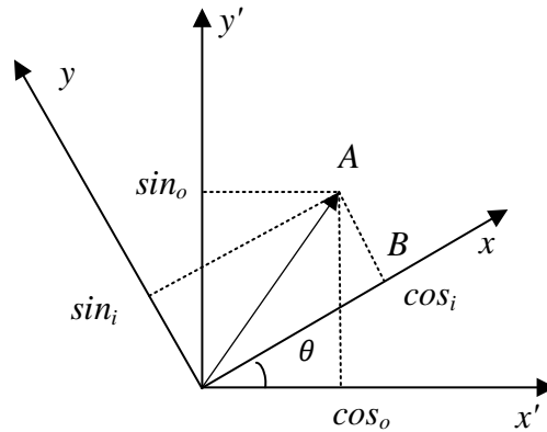
Figure 10-1 Coordinate Transformation
