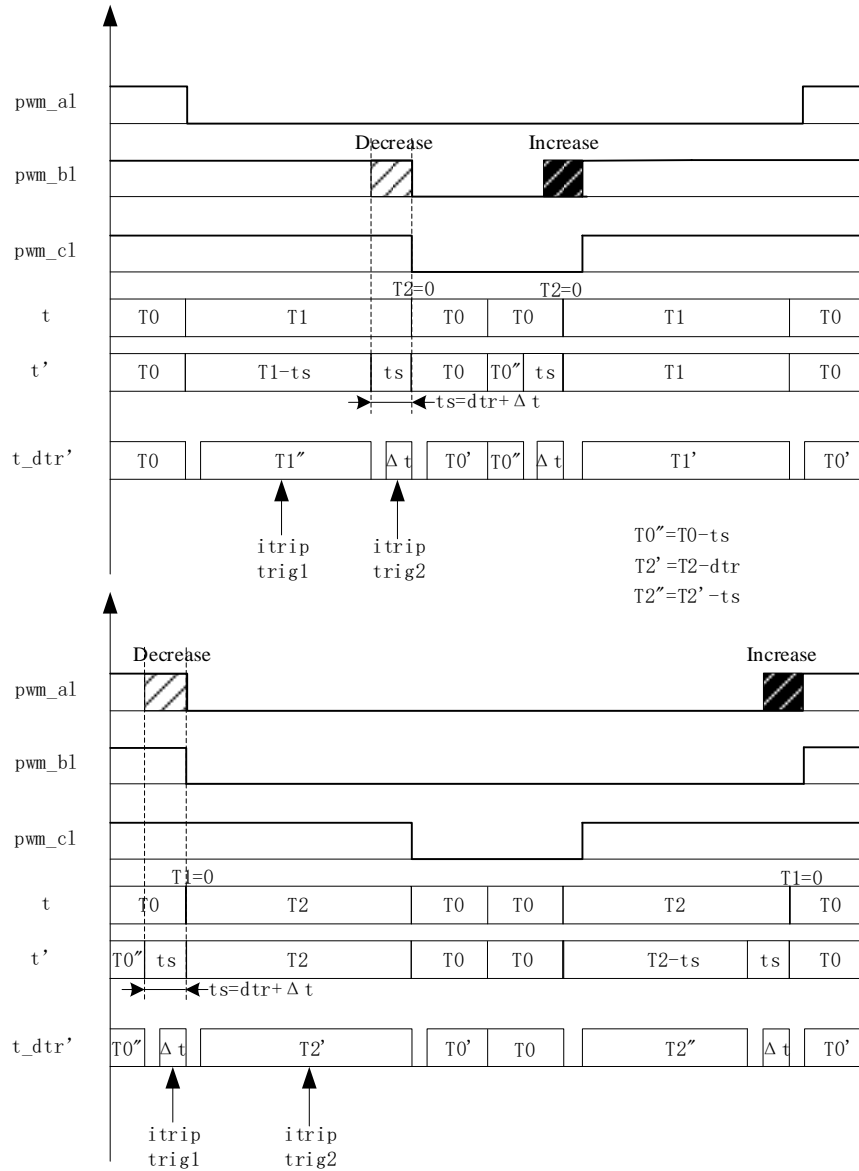
Figure 12-11 PWM Wave Shift in Single-shunt Current Sampling Mode
