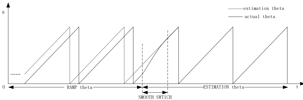
Figure 12-16 Angle Smooth Switching Waveform
