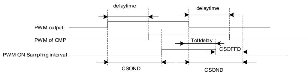
Figure 27-13 PWM ON Sampling Mode
