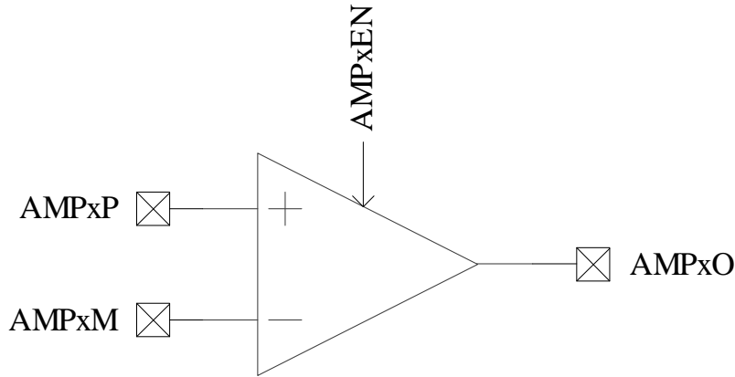
Figure 26-1 Schematic Diagram of Operational Amplifier module
