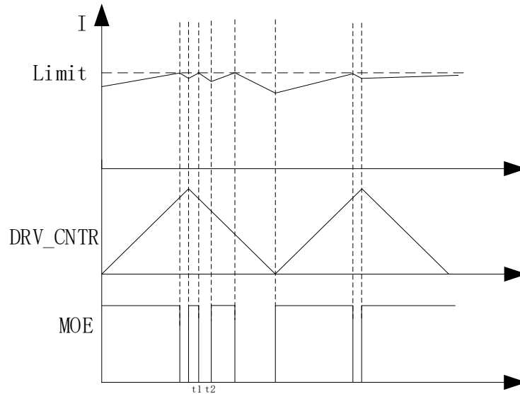
Figure 27-5 Cycle-by-Cycle Current Limiting Waveform ( t_2 - t_1 = 10\mu s ) when EVT\_FILT[MOEMD] = 10
