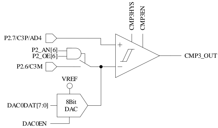
Figure 27-2 Single-comparator Input Mode
