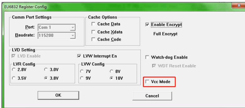
Figure 28-2 VCC_MODE Configuration
