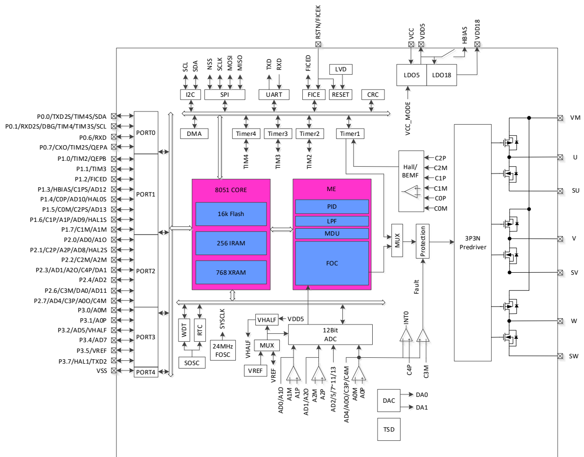
Figure 1-1 ES9650 Functional Block Diagram
