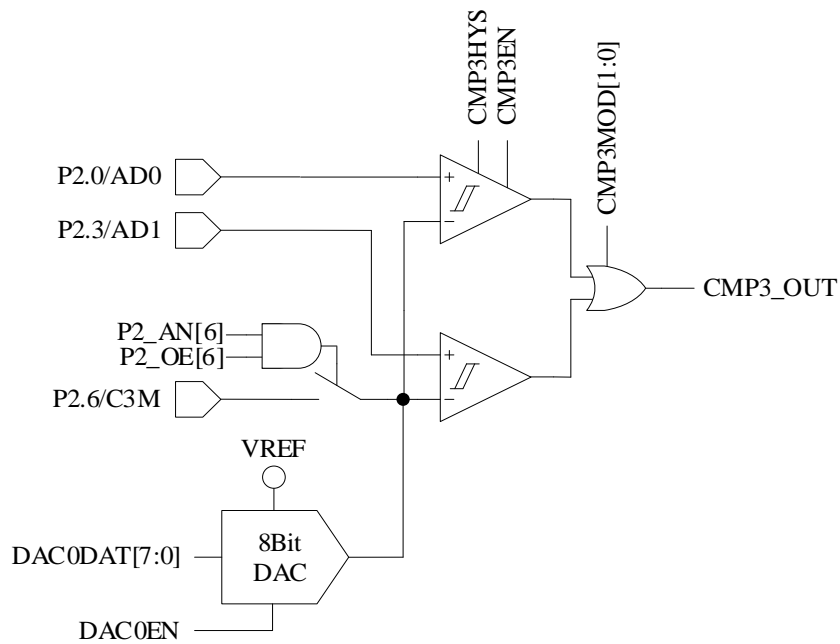
Figure 27-3 Dual-comparator Input Mode
