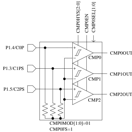
Figure 27-10 CMPG Mode with Built-in Three Comparators (with Functional Switching)
