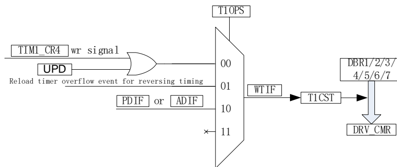
Figure 13-9 Block Diagram of Writing Sequence
