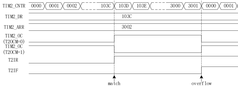
Figure 14-2 Output Mode Waveform
