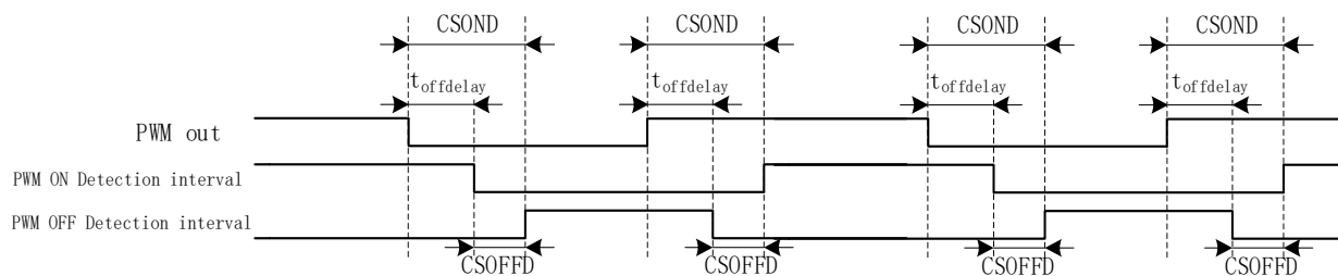
Figure 13-7 Timing Diagram of Sampling
