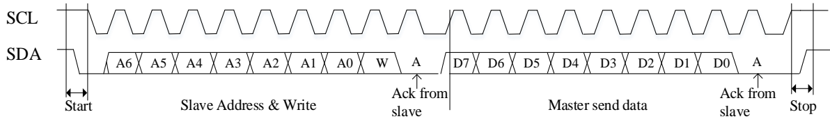
Figure 8-2 Master Sends Data to Slave
