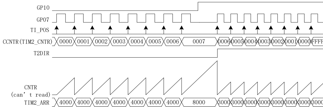
Figure 14-13 Timing Diagram of Step Mode
