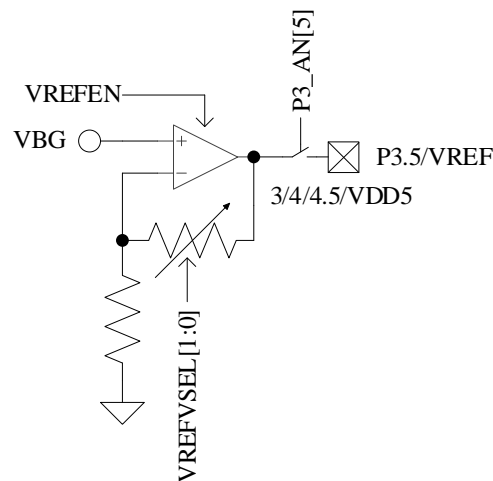
Figure 24-1 Diagram of VREF Module Input and Output
