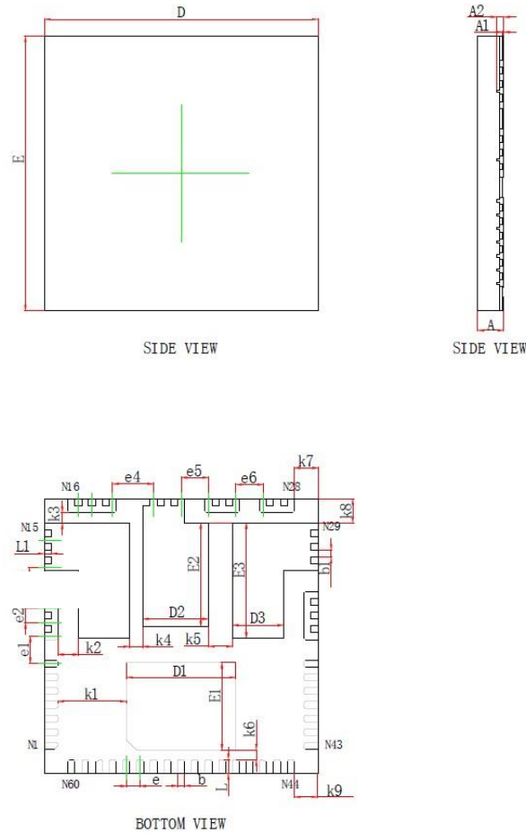
Figure 3-1 Package Dimensions of QHFBP8080-60L_8x8
