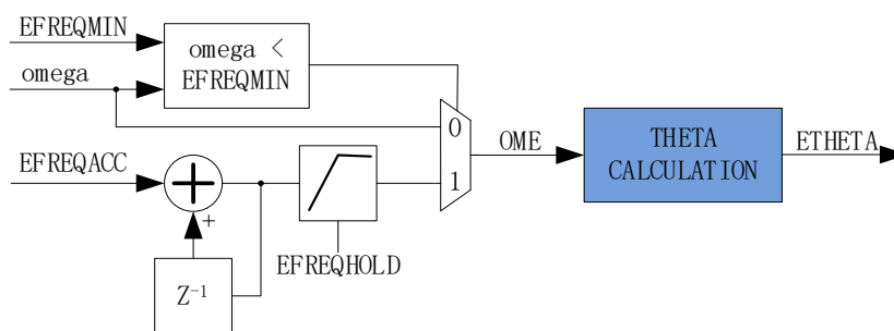
Figure 12-15 Schematic Block Diagram of Forced Angle of Estimator
