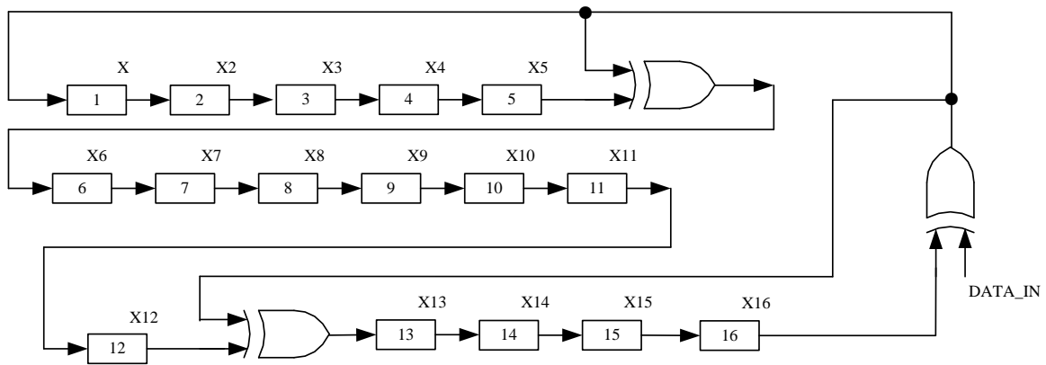
Figure 30-2 CRC16 Schematic Diagram
