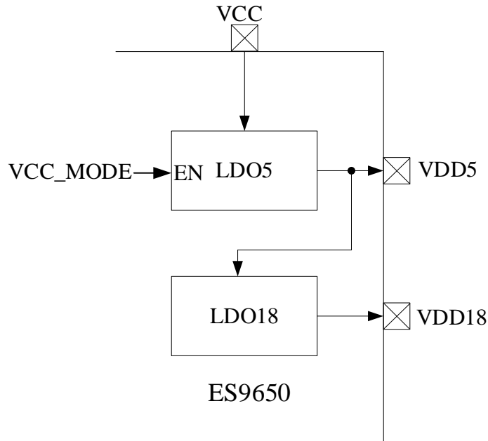
Figure 28-1 Functional Block Diagram of Power Supply
