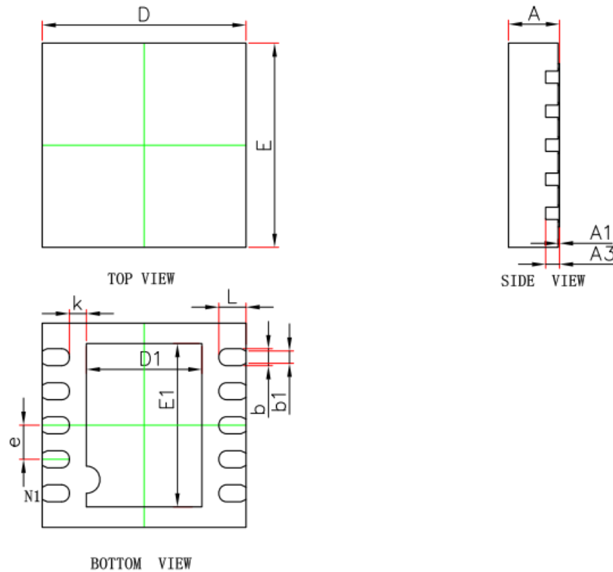
Figure 2-1 DFN10 Package Outline Dimensions
