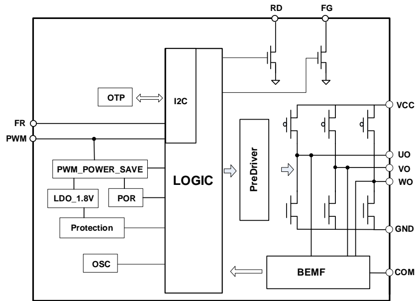
Figure 1-1 Functional Block Diagram of FT3206D
